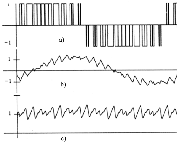
Figure 13.30 Computed waveforms for sinusoidal PWM scheme ( F_{nc} = 21 ), f = 60 Hz: a) line to line voltage V_{ab} , b) line current i_{ab} , c) developed torque
