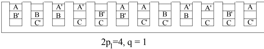
Figure 20.7 Triple-layer winding with chorded coils ( y/\tau = 2/3 ) (very short end connections)
