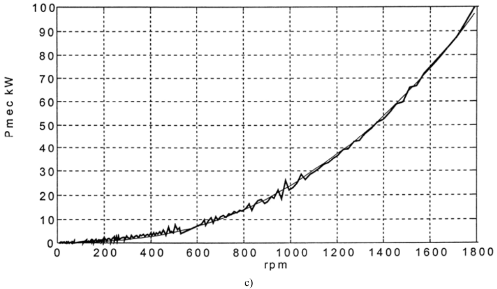
c) Figure 22.31 (continued): c) mechanical losses versus speed
