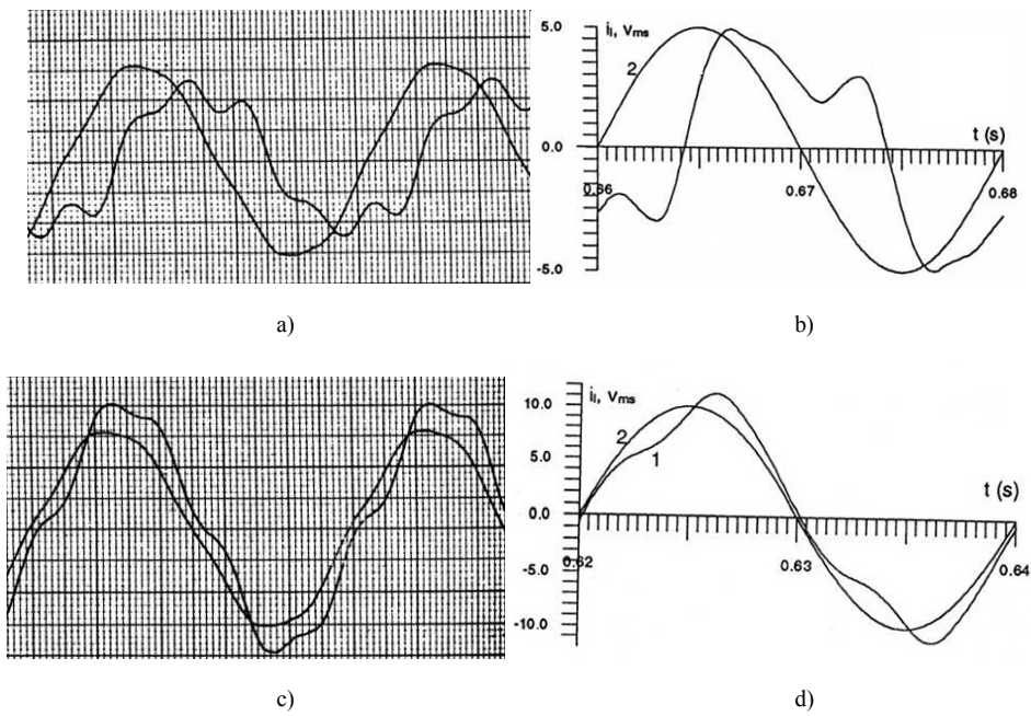
Figure 25.3 Steady state by the d-q model with saturation included: a) and b)- no-load c) and d)- on-load a) and c)- test results b) and d)- digital simulation
