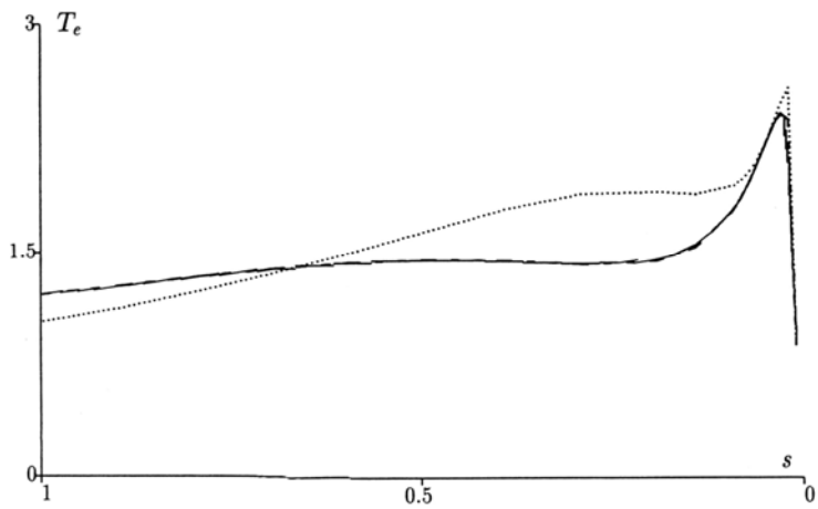
Figure 22.26 The static characteristic of electromagnetic torque T_e = f(S) : [22] — the theoretical characteristic of T_e = f(S) ..... – the characteristic calculated for starting values of parameters ----- – the characteristic calculated for final values of estimated parameters
