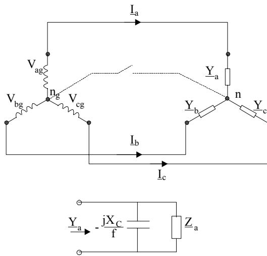
Figure 19.15 Star-connected SEIG
