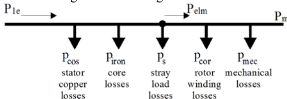
Figure 7.7 Power balance for motoring operation
