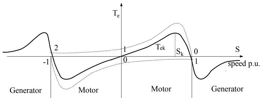
Figure 24.3 Torque/speed curve for open auxiliary winding (single-phase winding operation)
