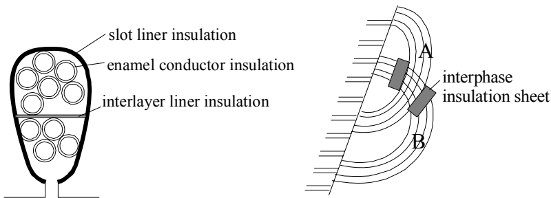
Figure 3.7 Random-wound coils insulation
