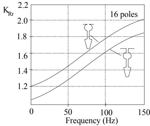
Figure 9.17 End ring skin effect resistance coefficient K_{Rr}
