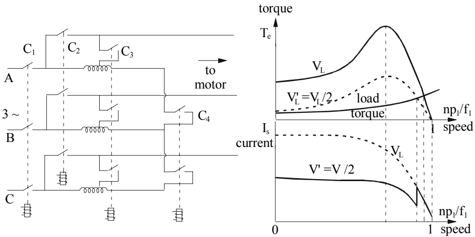
Figure 8.2 Autotransformer starting
