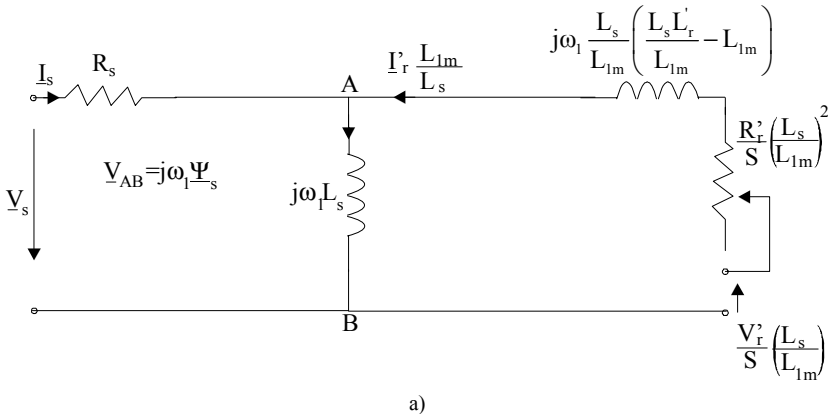
Figure 7.25 Equivalent circuit (continued): a) with stator flux shown,
