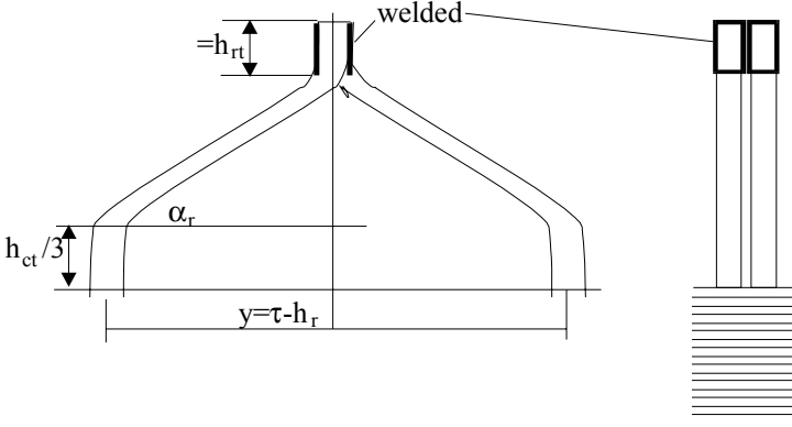
Figure 16.17 Rotor half-formed coil winding
