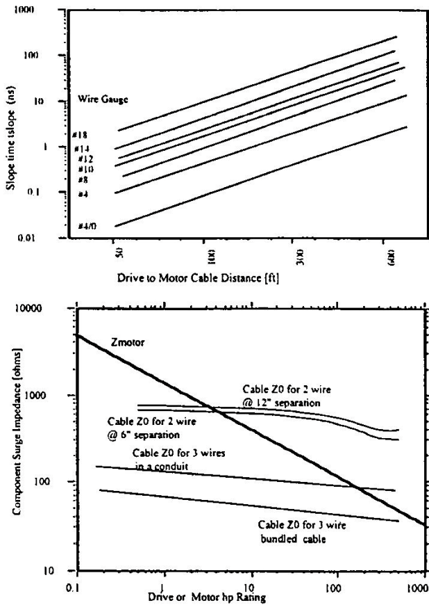
Figure 21.4 Differential mode impedance ( Z_m )
