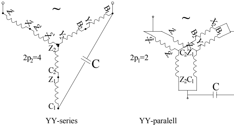
Figure 4.22 4/2 pole two-phase winding for single-phase supply made from a three-phase winding
