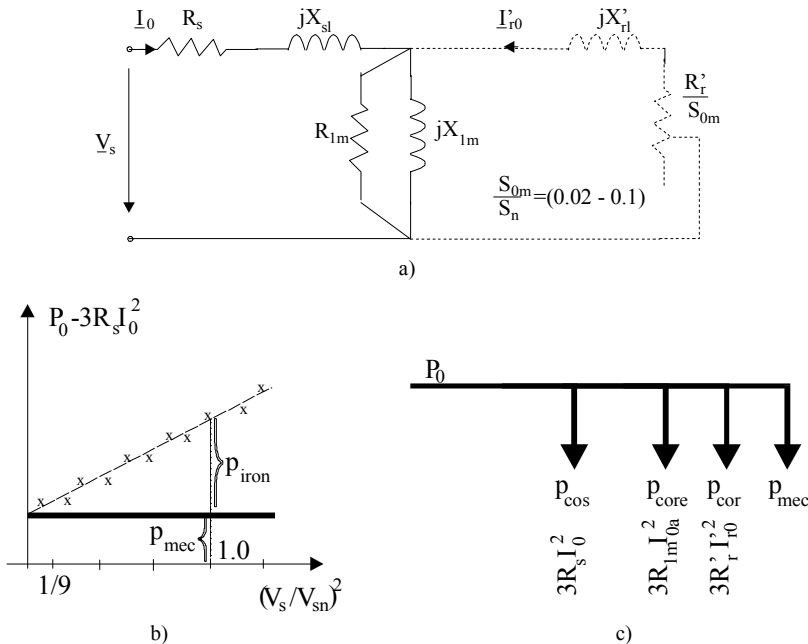
Figure 7.5 No-load motor operation (continued): a) equivalent circuit, b) no-load loss segregation, c) power balance,
