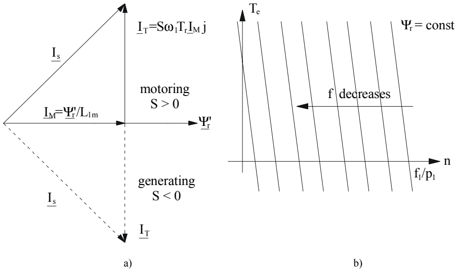
Figure 8.16 Rotor flux vector control: a) stator current components, b) torque versus speed curves for variable frequency f_l at constant rotor flux
