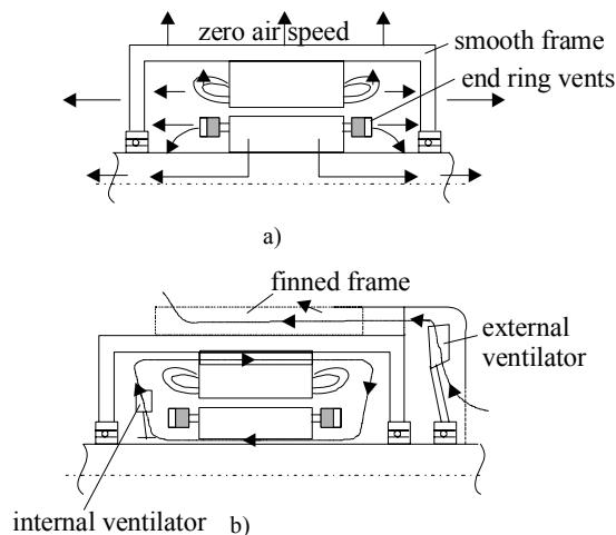
Figure 12.2 Cooling methods for induction machines (continued):
