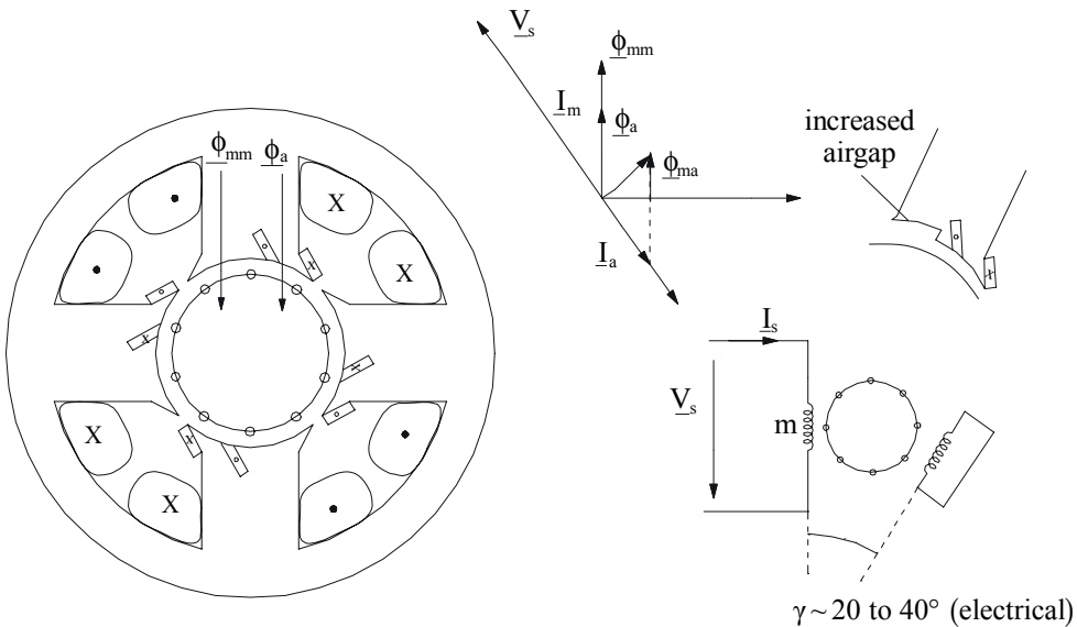
Figure 23.11 The shaded-pole induction motor
