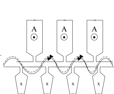
Figure 9.3 Zig-zag flux lines
