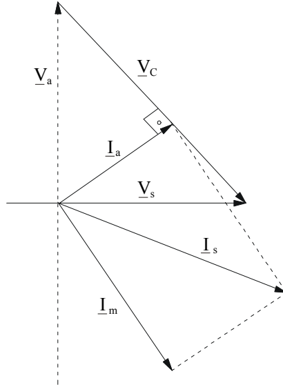
Figure 24.7 Phasor diagram for S = 0.06 , C = 4 \mu F and the data of Example 24.2
