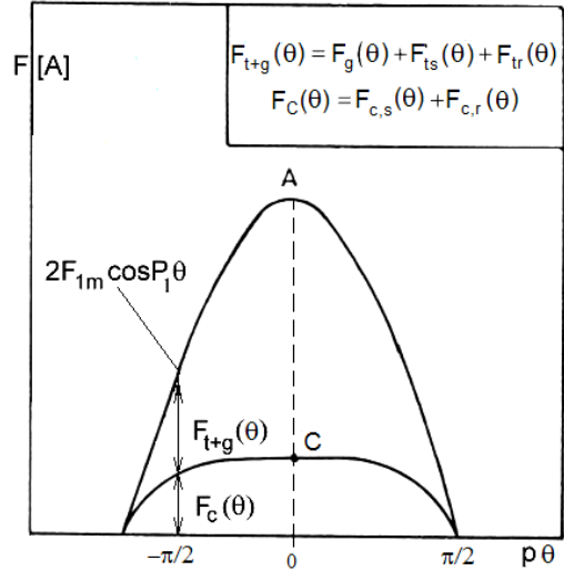
Figure 5.17 Mmf – total and back core component F
