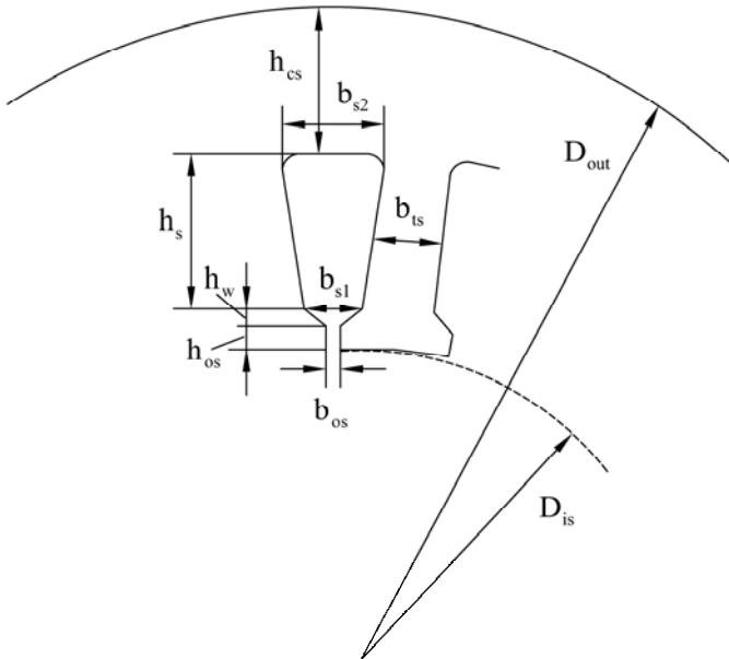
Figure 15.5 Stator slot geometry
