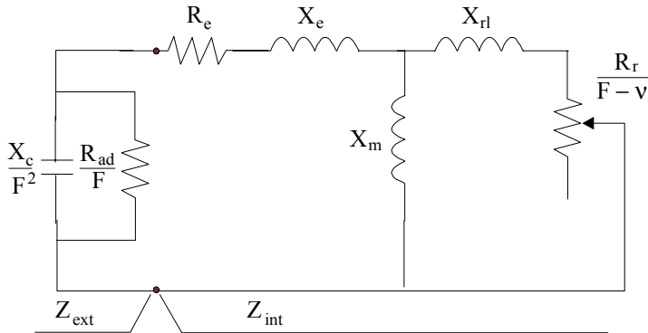
Figure 13.40 Additional resistance R_{ad} for preventing SSR
