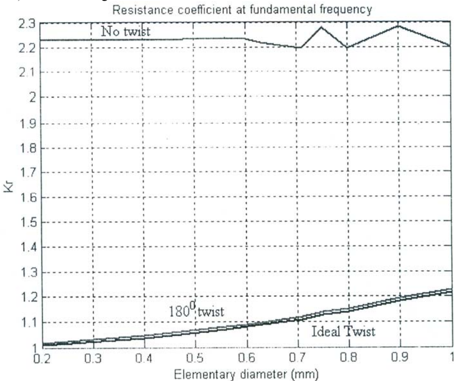
Figure 9.35 Resistance a.c. factor K_r for 2333 Hz with 18 layer single turn coil without twisting.
