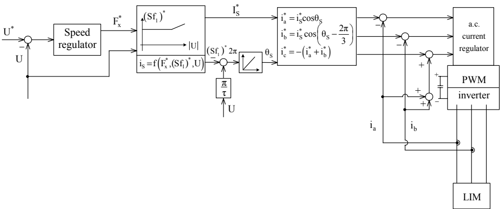
Figure 20.33 Generic slip frequency (Sf_1) control of LIM for propulsion only
