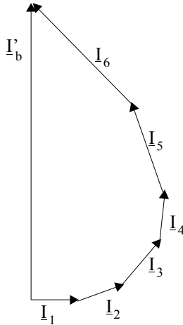
Figure 9.14 Layer currents and the bar current with skin effect
