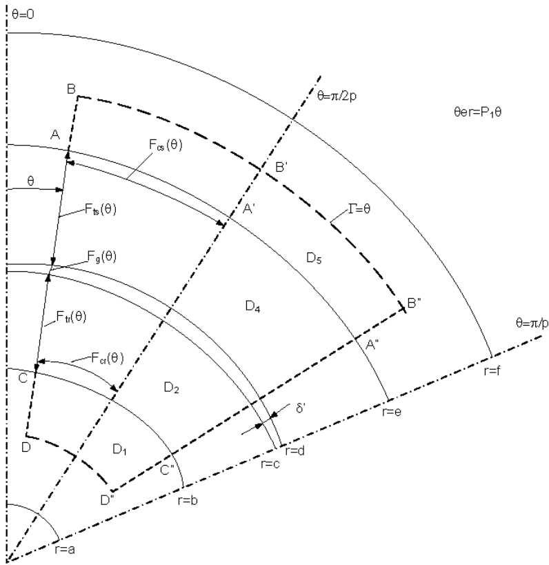
Figure 5.16 Ampere’s law contours
