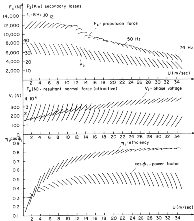
Figure 20.31 Motoring performance
