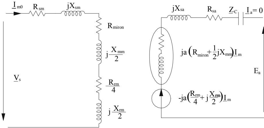
Figure 28.3 Simplified no-load ( S = 0 ) equivalent circuit with series core loss resistance R_{miron} in both circuits (the auxiliary winding is open)
