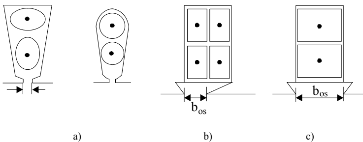
Figure 2.3 Slot geometrics to locate coil windings:
