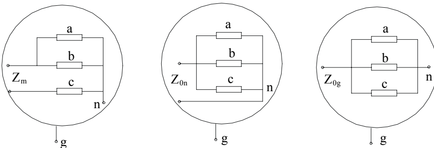
Figure 21.3 Line ( Z_m ) neutral ( Z_{on} ) and ground (common mode Z_{0g} )
